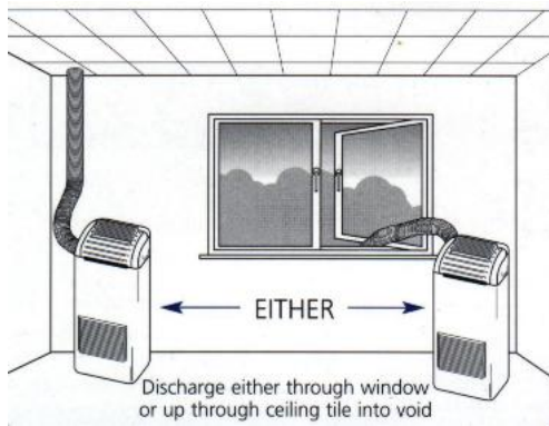
KY.35 - Installation Options
